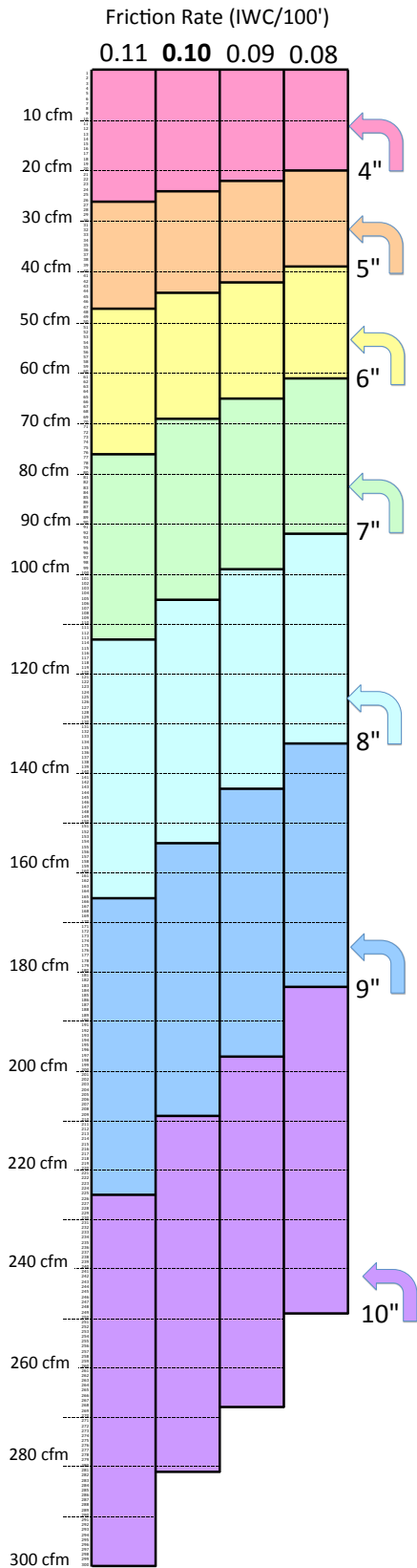
Flex Duct Sizing Table (C) 2020, Russell King, M.E.
